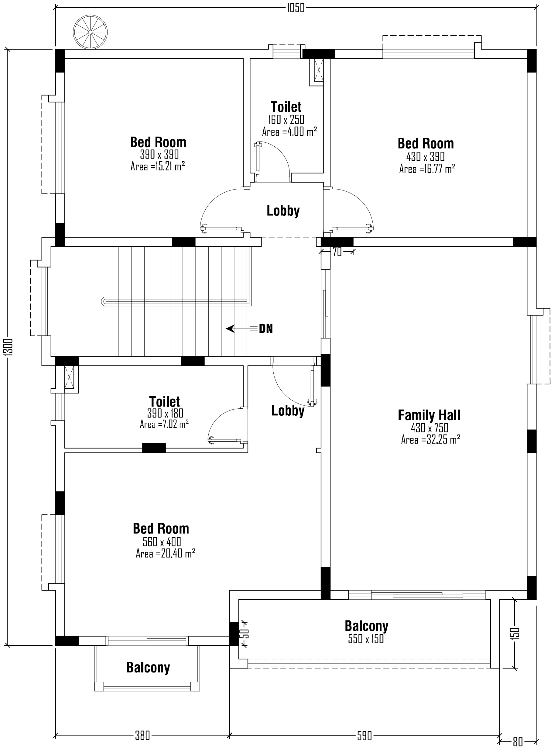
FIRST FLOOR PLAN AREA= 141.79sqm
