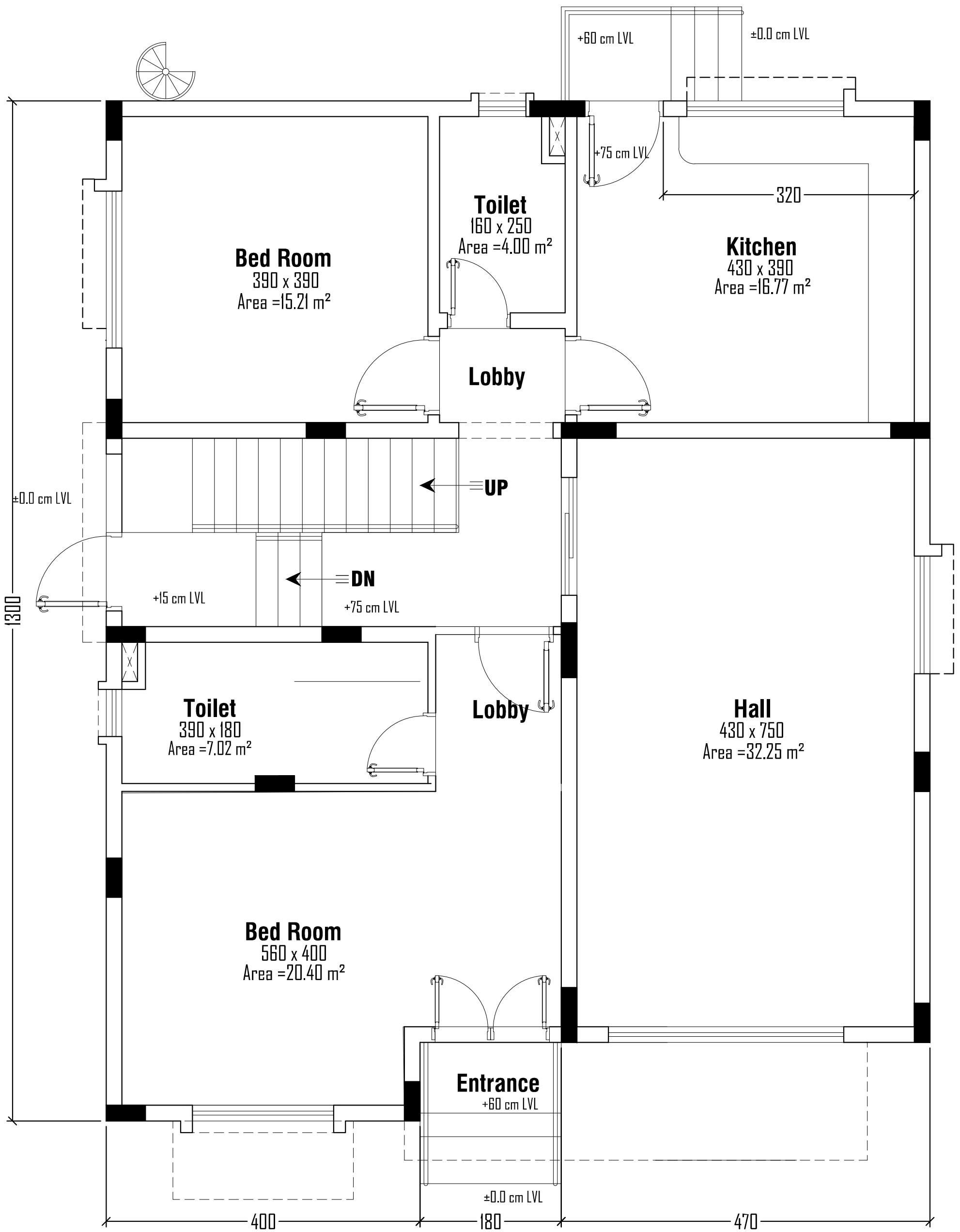
GROUND FLOOR PLAN AREA= 131.62sqm
