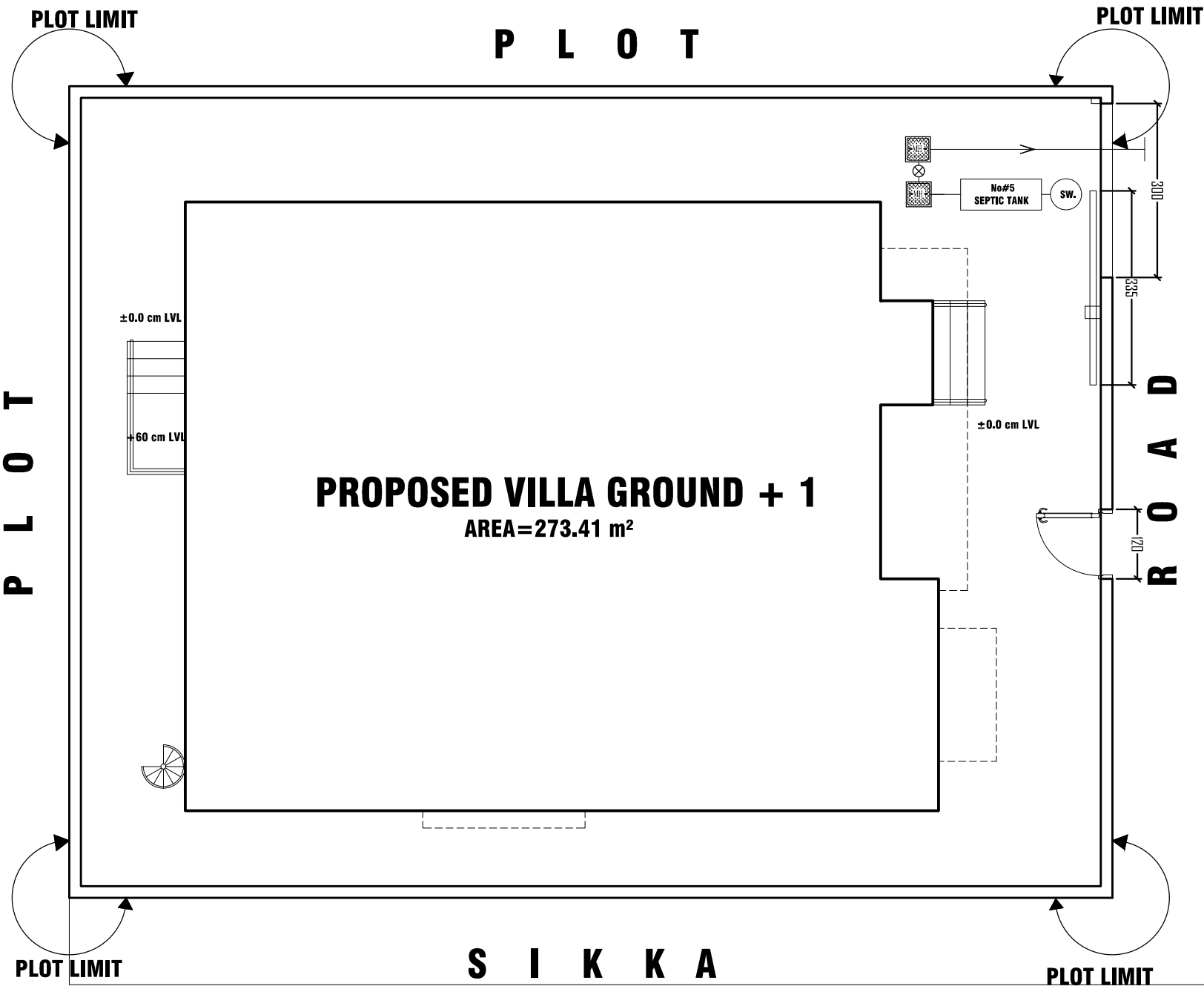
SETTING OUT PLAN SCALE - 1 : 100
